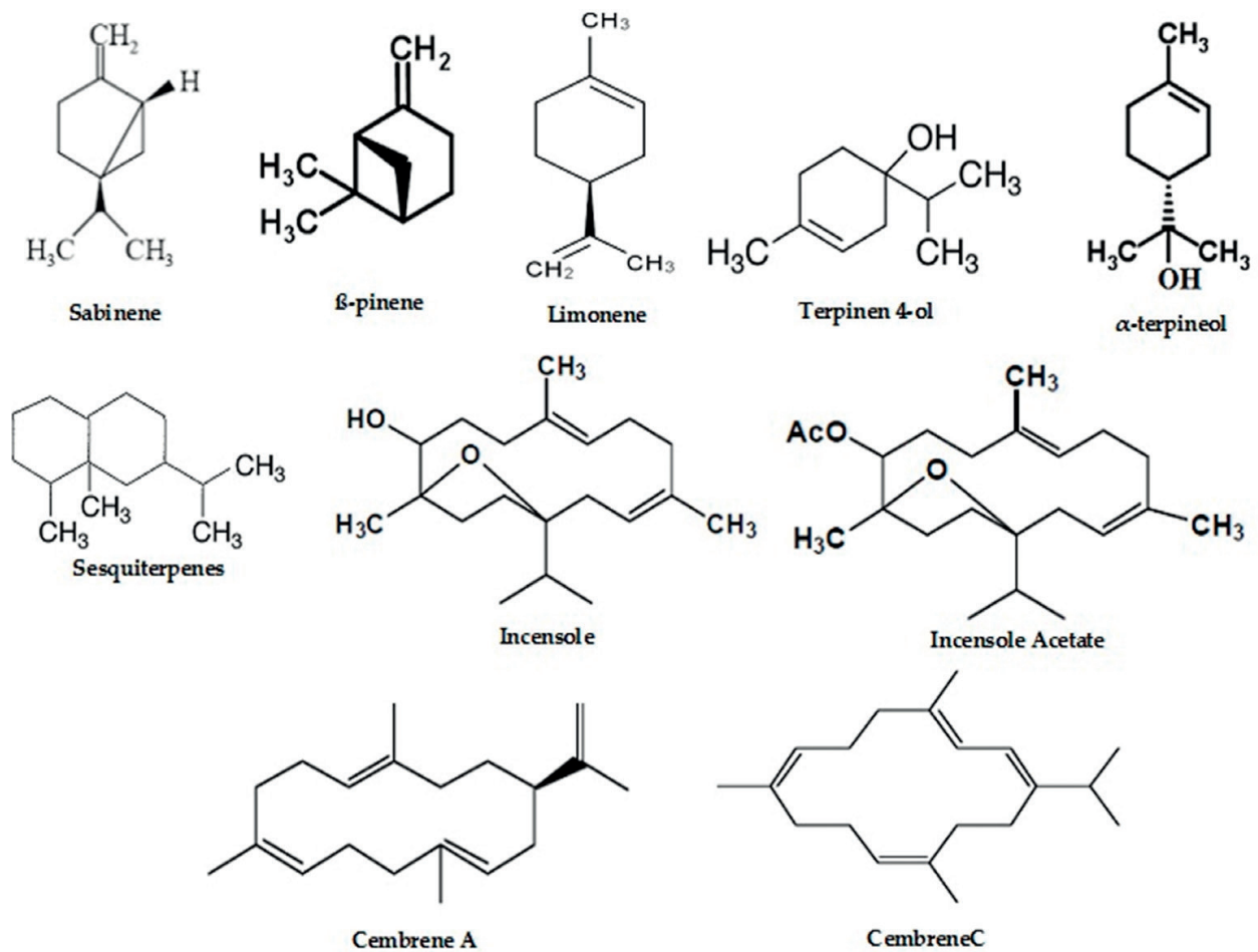
Figure 2. Chemical structures of doom fruit essential oil.
