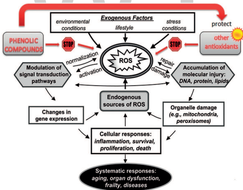
Figure 6. The scheme of factors involved in the formation of free radicals and a cellular response to reactive oxygen species (ROS). The red arrow and the text in red emphasize the importance of phenolic compounds, other reactive oxygen species (ROS). The red arrow and the text in red emphasize the importance of phenolic compounds, other antioxidants and the relationship between them. The sun signifies protection of other antioxidants by phenolic compounds.
