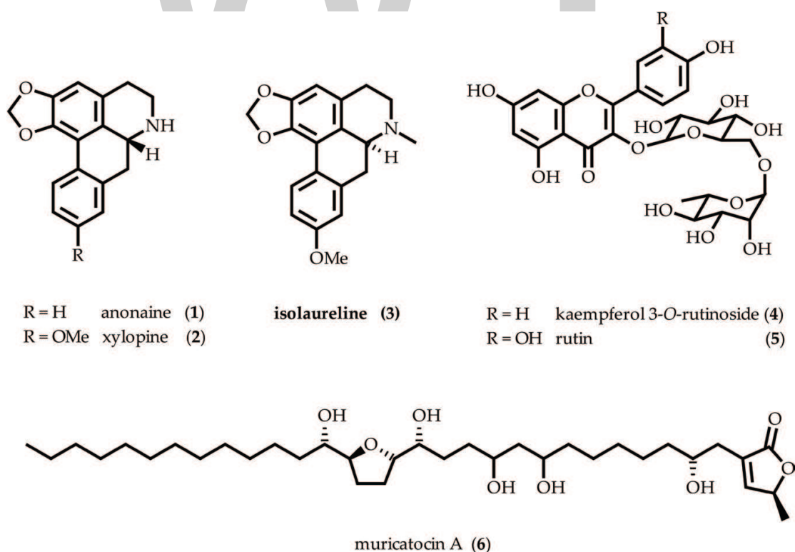
Figure 2. Molecules with FOXO1 inhibition activity isolated from Ammonia muricata [14].
