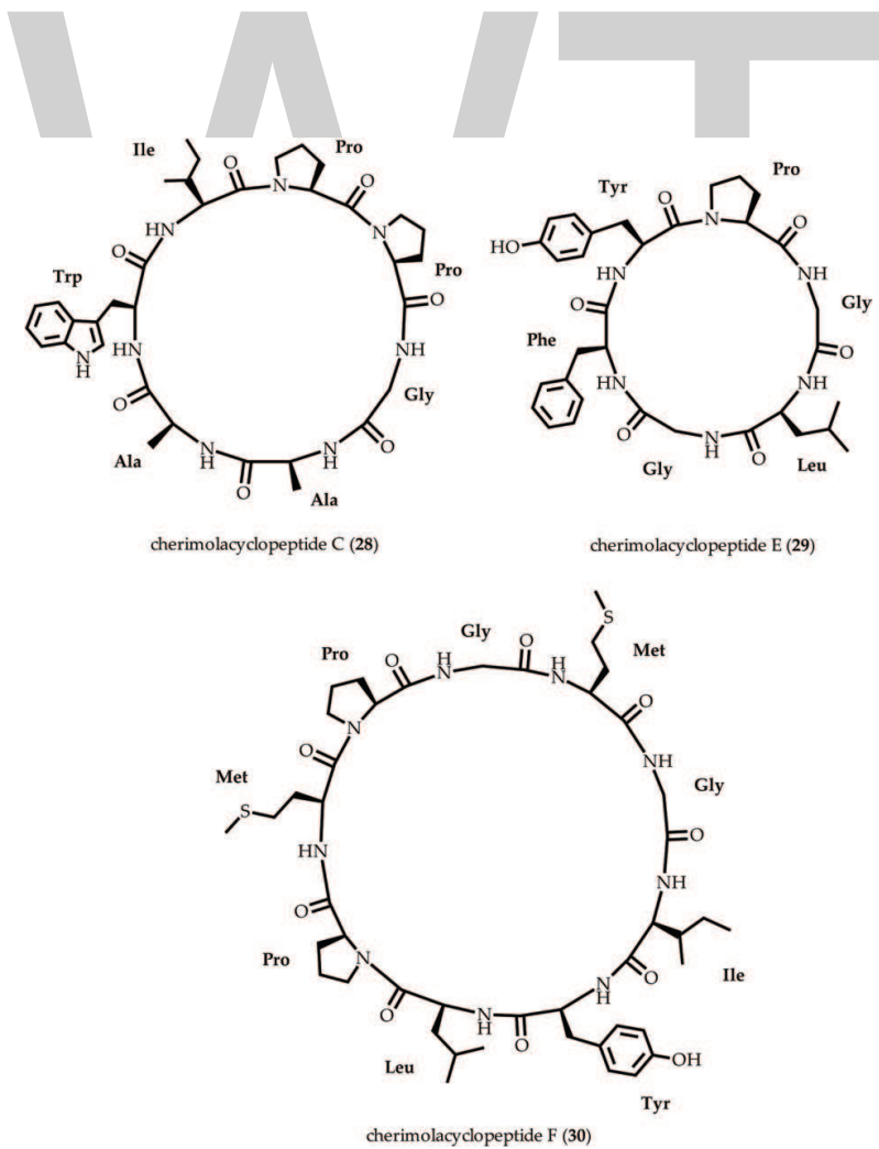
Figure 10. Cyclopeptides with anticancer activity isolated from the seeds of A. cherimola [54].
