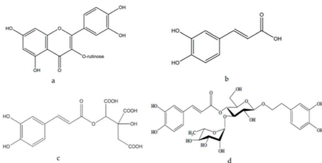
Figure 4. Structures of phytochemicals (a) quercetin-3-O-rutinoside, (b) caffeic acid, (c) Caffeoyl-hydroxycitric acid, and (d) verbascoside.
