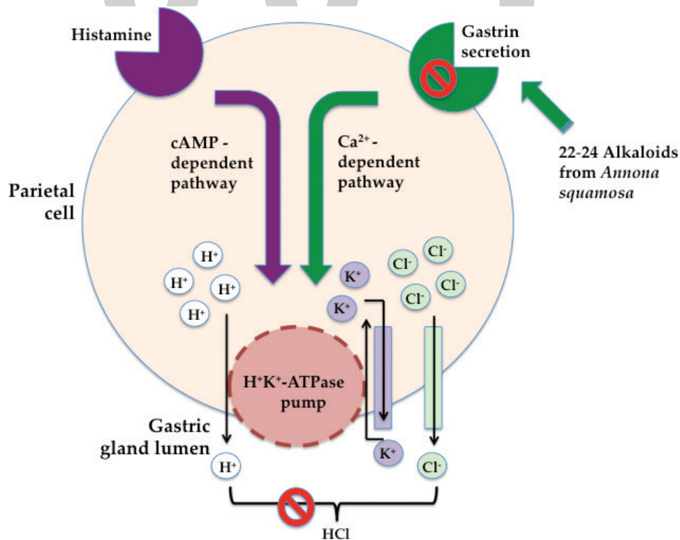
Figure 7. Inhibition of \text{H}^+\text{K}^+ -ATPase activity by alkaloids 22-24 from EtOH extracts of A. squamosa twigs.
